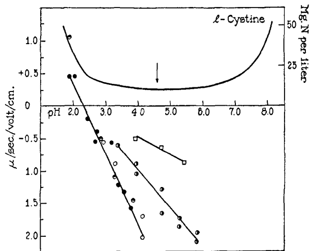
FIG. 5. The electric mobilities of cystine crystals suspended in hydrochloric acid and in sodium acetate buffers. The arrow points to the isoelectric point of dissolved cystine. ● ◐ ○, hydrochloric acid; ◐, N/200 sodium acetate; ◑, N/200 sodium acetate + N/5 sodium chloride. Smooth curve, solubility (Sano).
